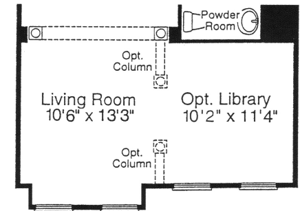
OPTIONAL FIRST FLOOR PLAN
