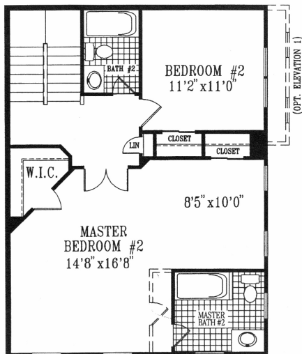
ALTERNATE SECOND FLOOR PLAN W/OPT. DUAL MASTER BEDROOMS
