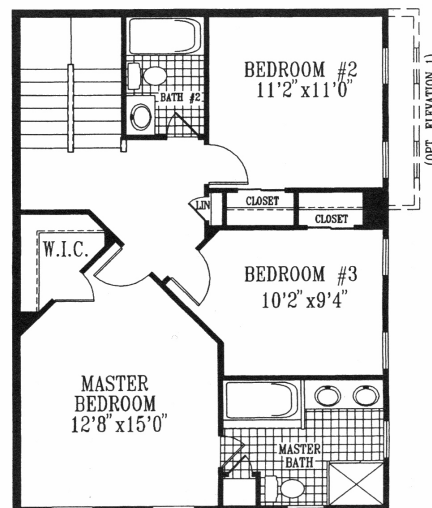
ALTERNATE SECOND FLOOR PLAN W/OPT. LOFT STUDY
