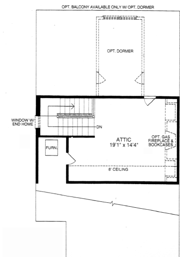
OPT. ATTIC PLAN
