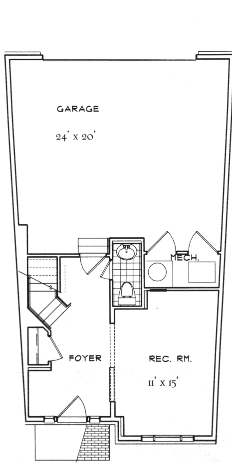
FIRST LEVEL
