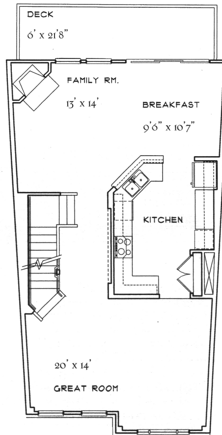
MAIN LEVEL
